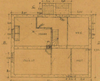
2d. Plan.
